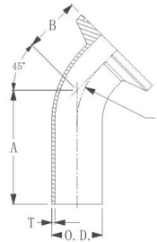
DT-4.1.1-5 单卡45度弯头 Automatic Tube Weld: Hygienic Clamp Joint, 45-deg Elbow
