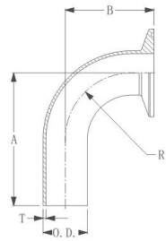
DT-4.1.1-2 单卡90度弯头 Automatic Tube Weld: Hygienic Clamp Joint, 90-deg Elbow
