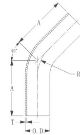
DT-4.1.1-4 焊式45度长弯头 Automatic Tube Weld: 45-deg Elbow
